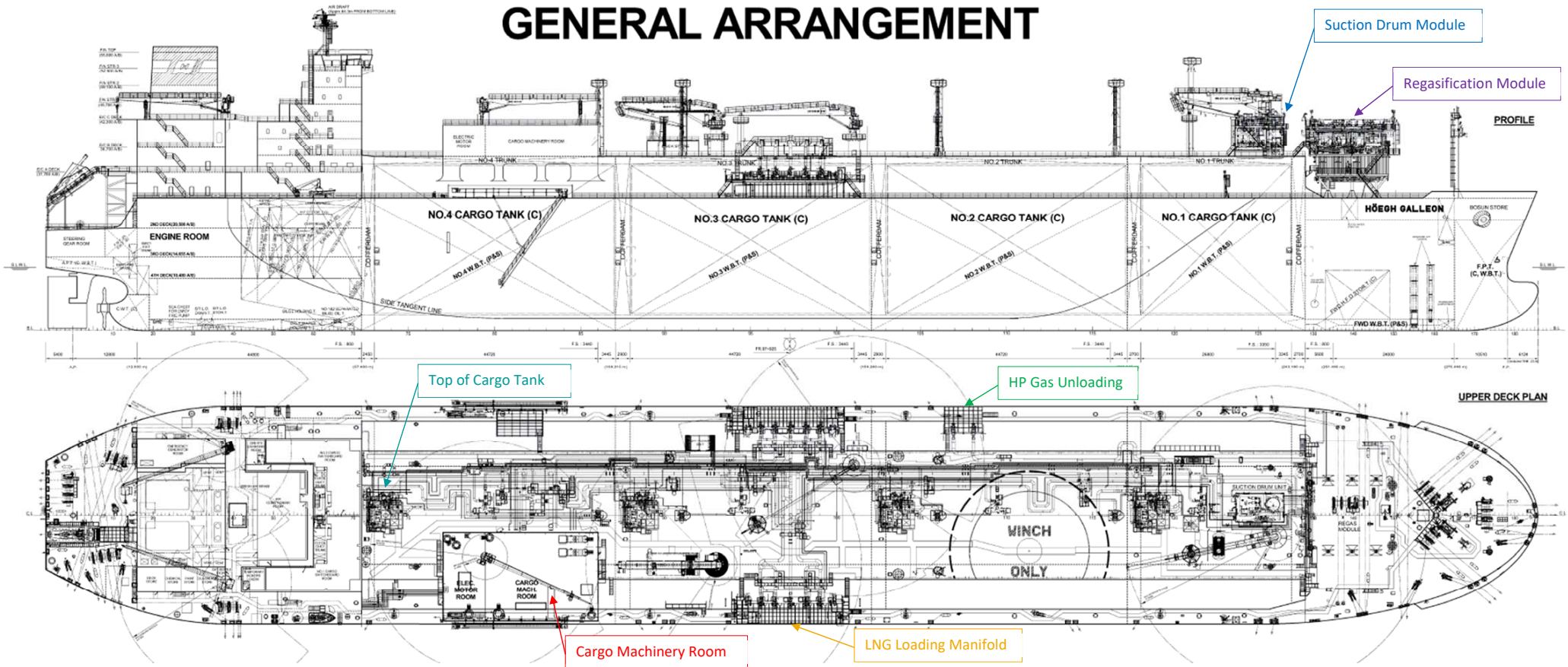
Figure 3-4: FSRU General Arrangement
